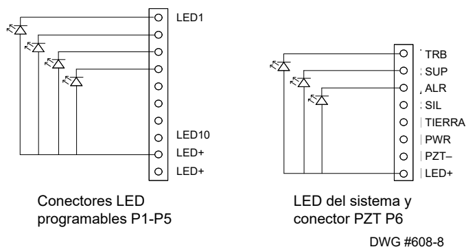
Figure 26. Conectores DRV-50 "P1-P5" y "P6"
