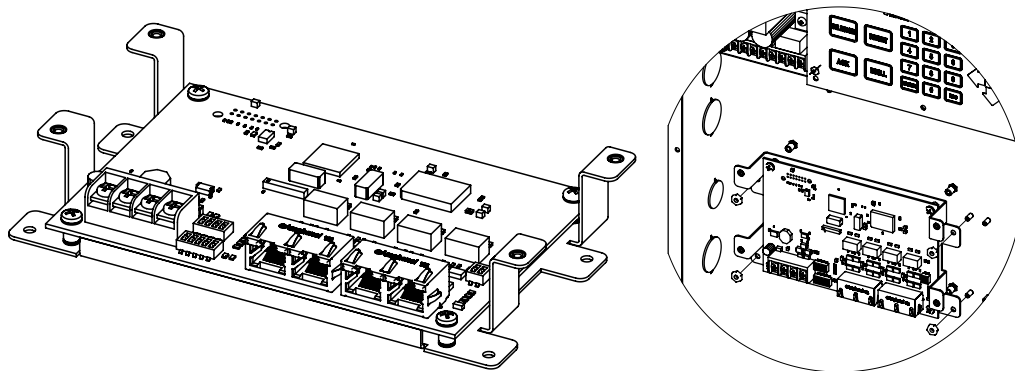
Figure 38. Tarjeta de red NCE-1000
