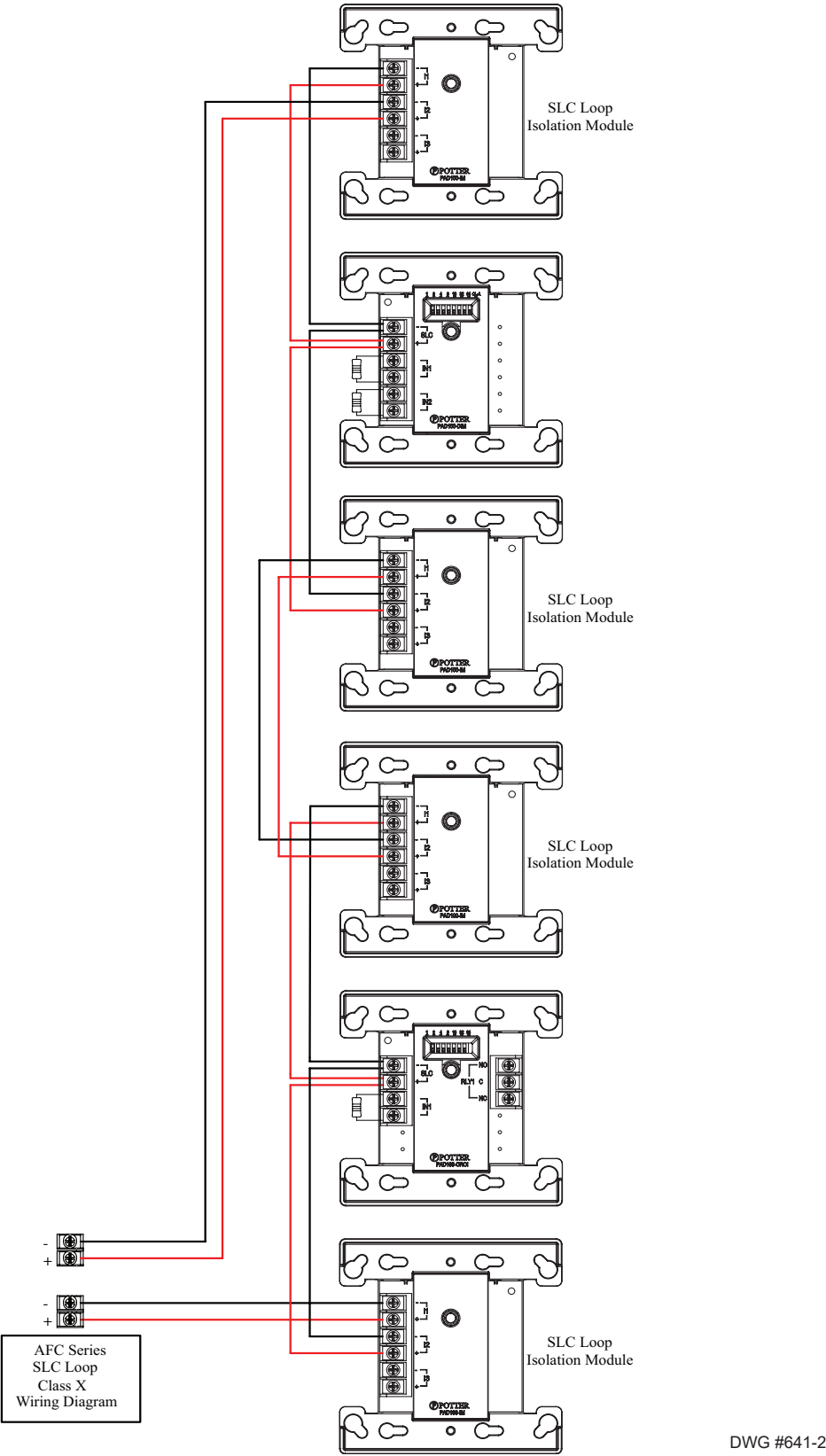
Figure 8. PAD Protocol Class X Showing PAD100-IMs Installed
