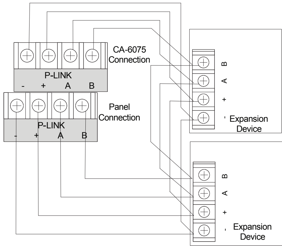
DWG #602-12A
