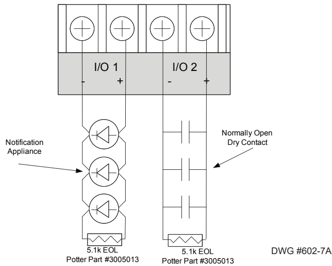
Figure 7. I/O Circuits Shown as Class B NAC / Dry Contact Input
