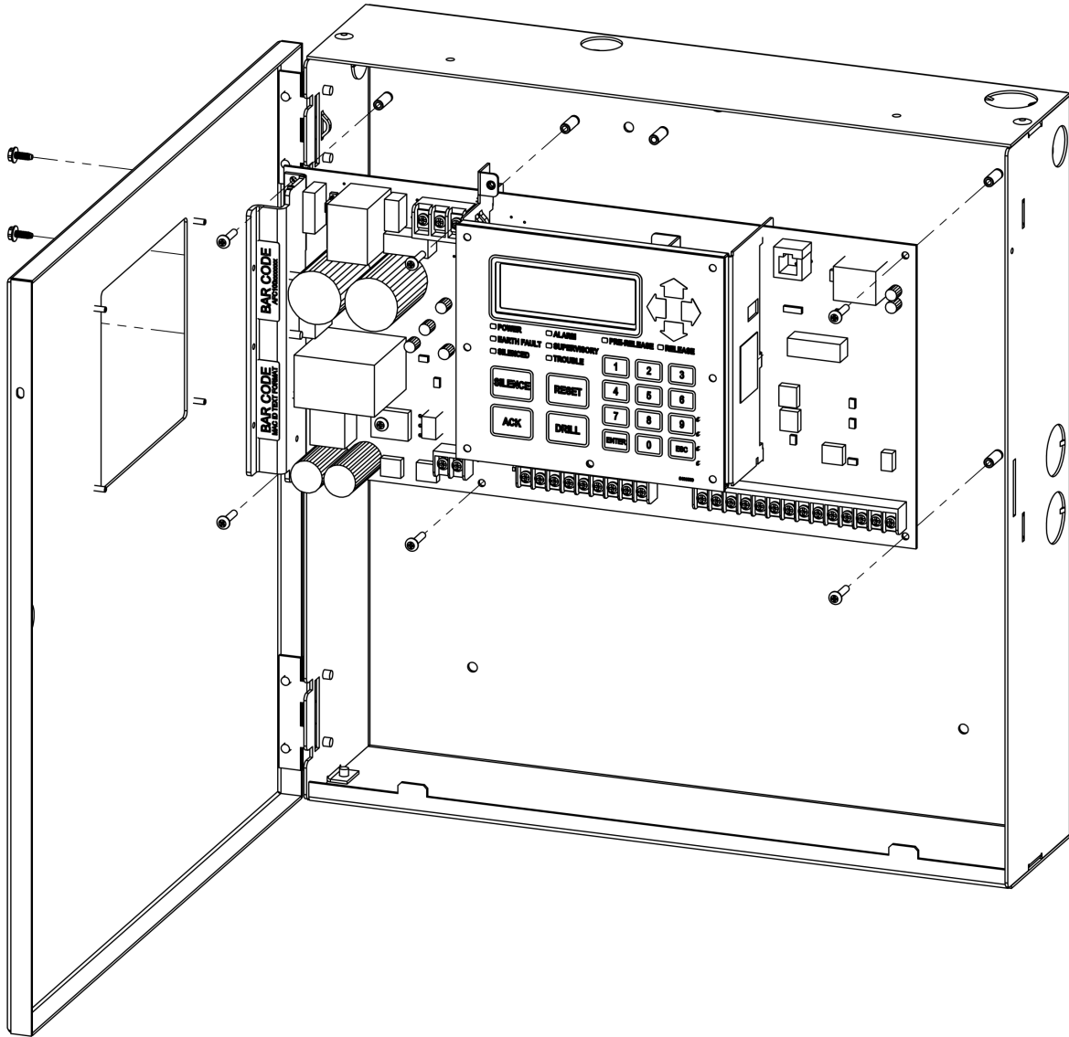
Figure 40. AFC-50 Cabinet Showing Circuit Board Assembly
