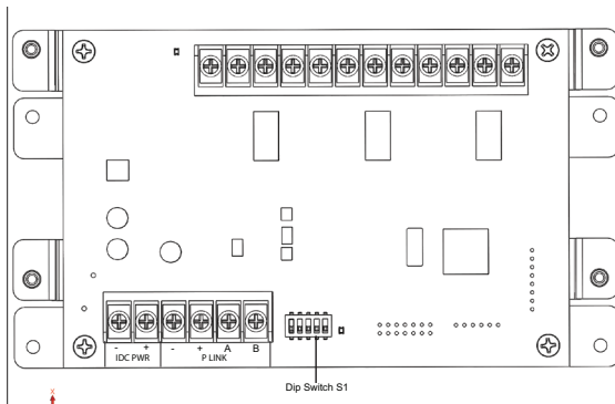
Figure 35. IDC-6 Initiating Device Circuit Expander and IDC-6 Installation
