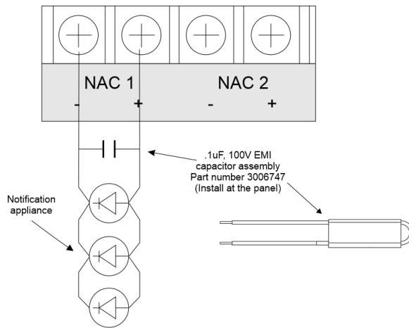
Figure 6. NAC EMI capacitor assembly wiring diagram
