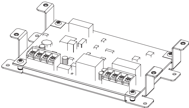
Figure 22. PAD100-SLCE / SLCE-127 Board & Showing Mounting Bracket
